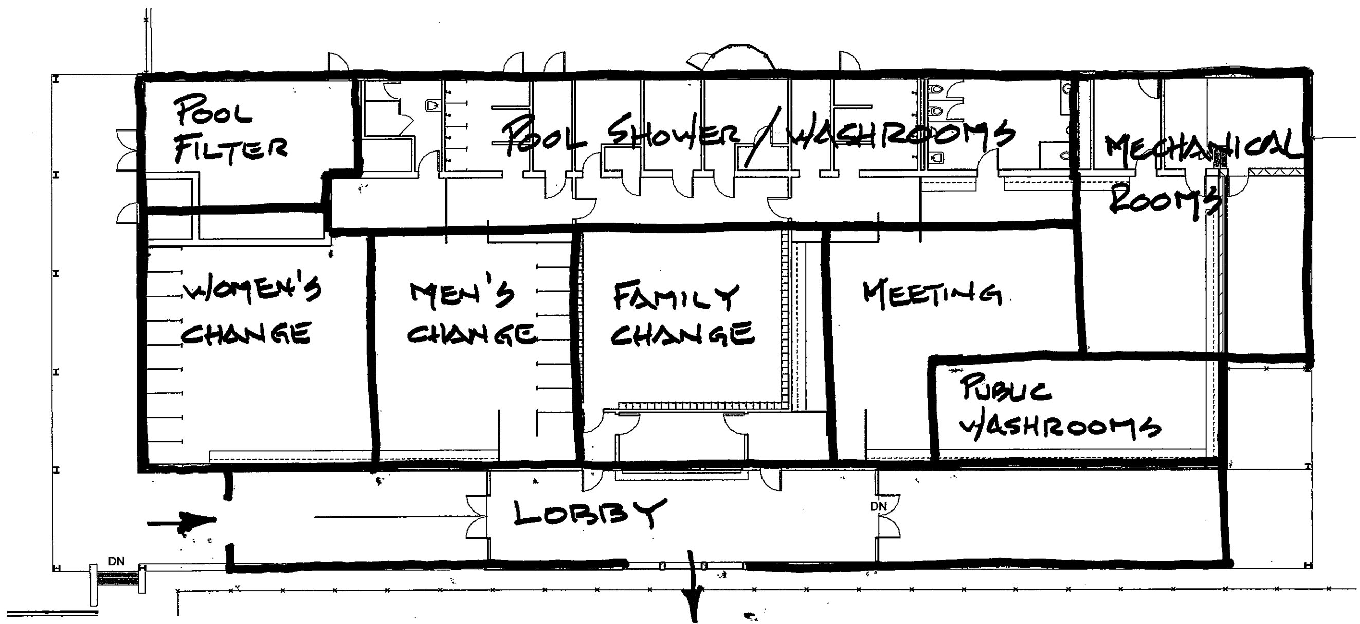
1 EXISTING GROUND FLOOR PLAN P-103 1:150
